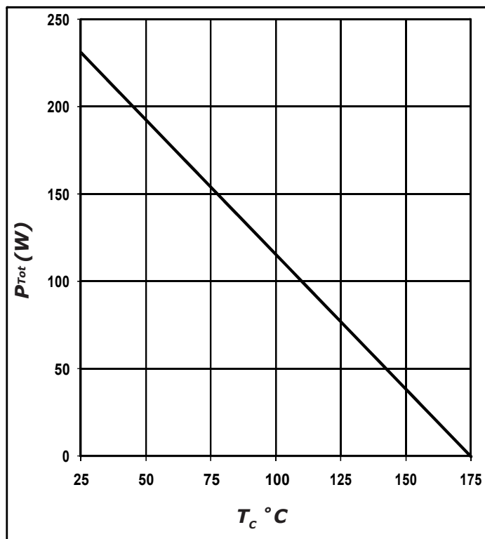
Figure 4. Power Derating
