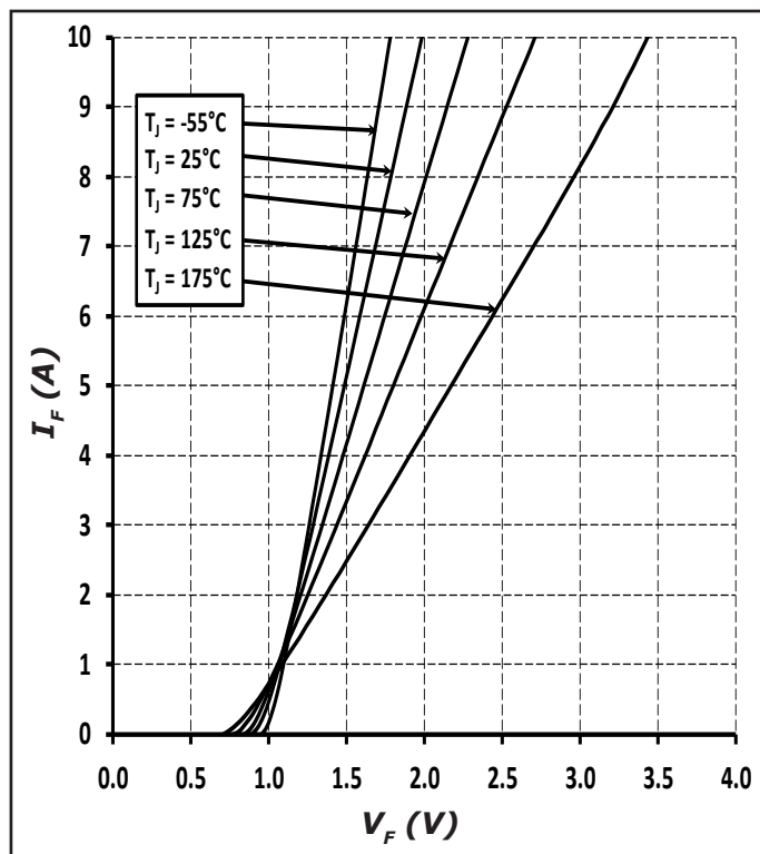
Figure 1. Forward Characteristics
