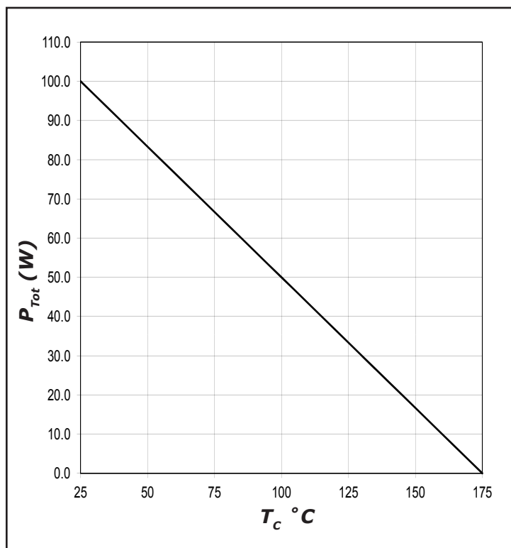
Figure 4. Power Derating
