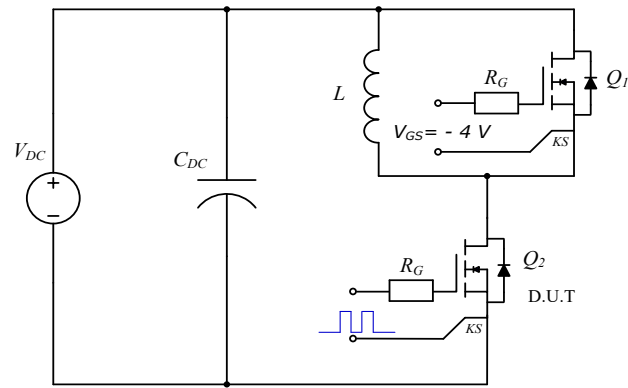
Figure 29. Clamped Inductive Switching Waveform Test Circuit
