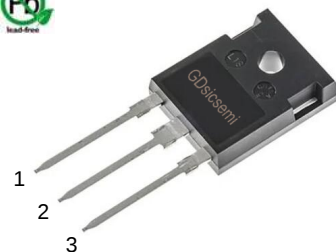
TO-247-3
